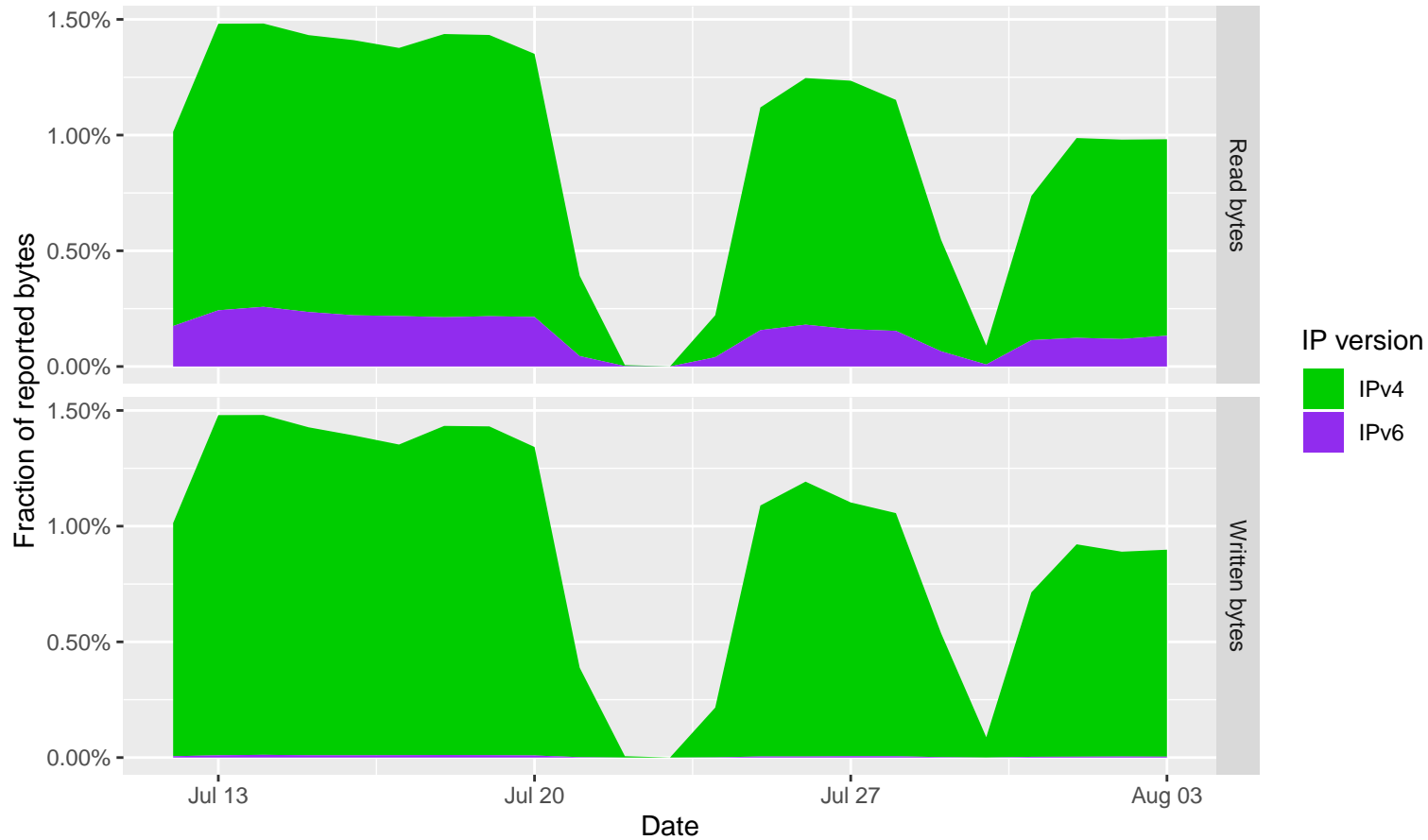
Fraction of reported bytes for which IP version is known
